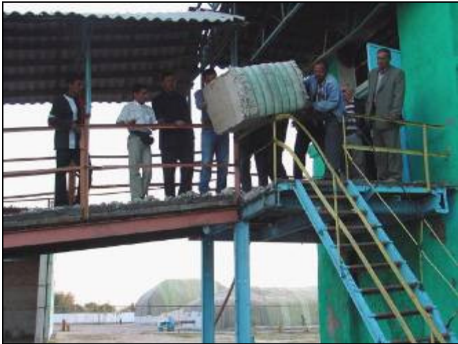
Fall test from a height of 4 m
